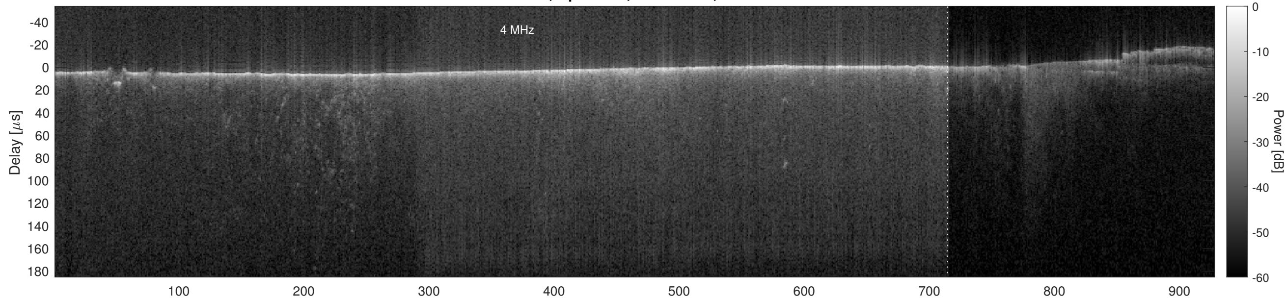
Orbit 3729, Optimized, No Window, Channel 2
