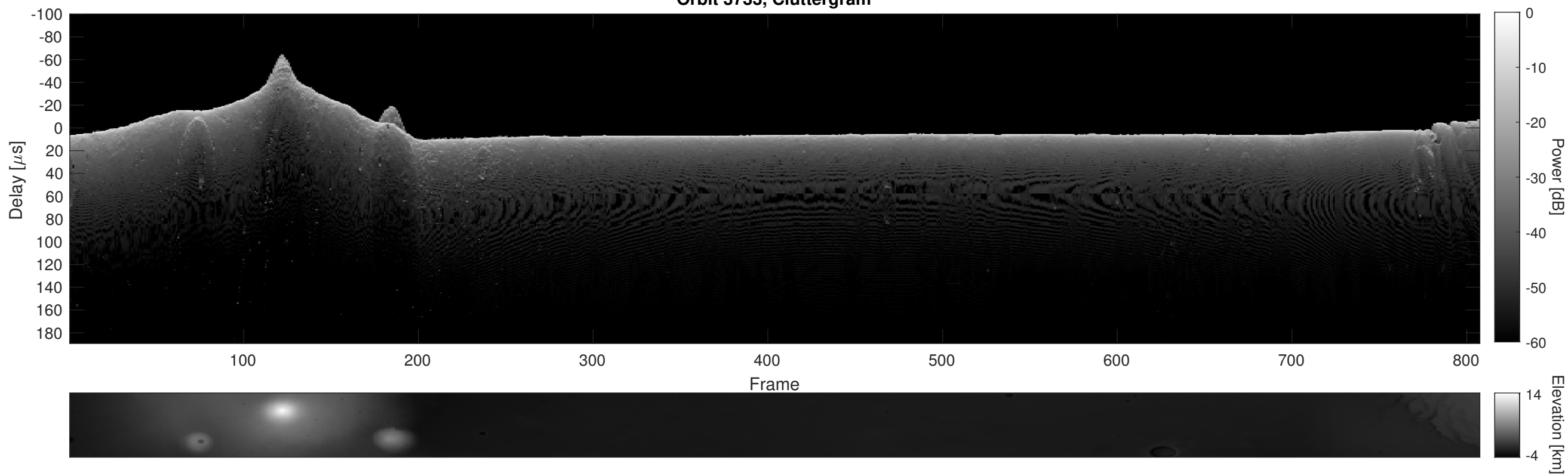
Orbit 3733, Cluttergram
