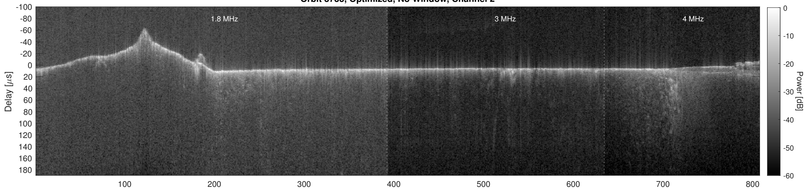
Orbit 3733, Cluttergram
