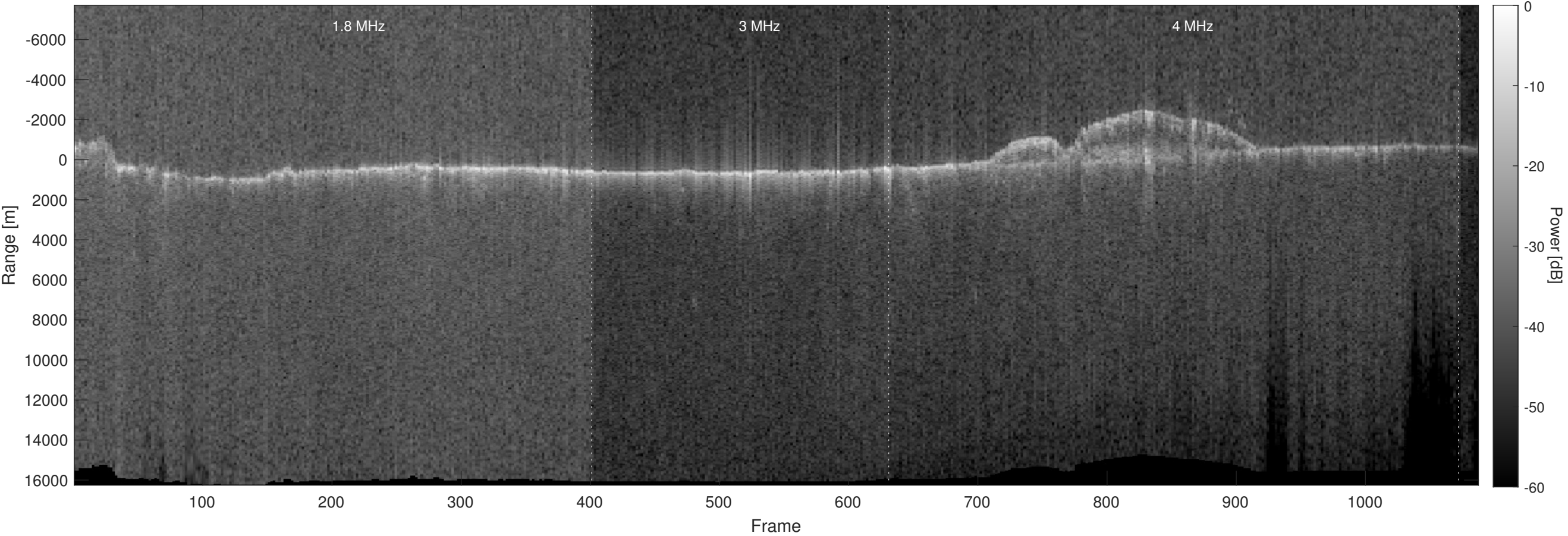
Orbit 3735, Optimized, No Window, Depth-Corrected, Channel 2
