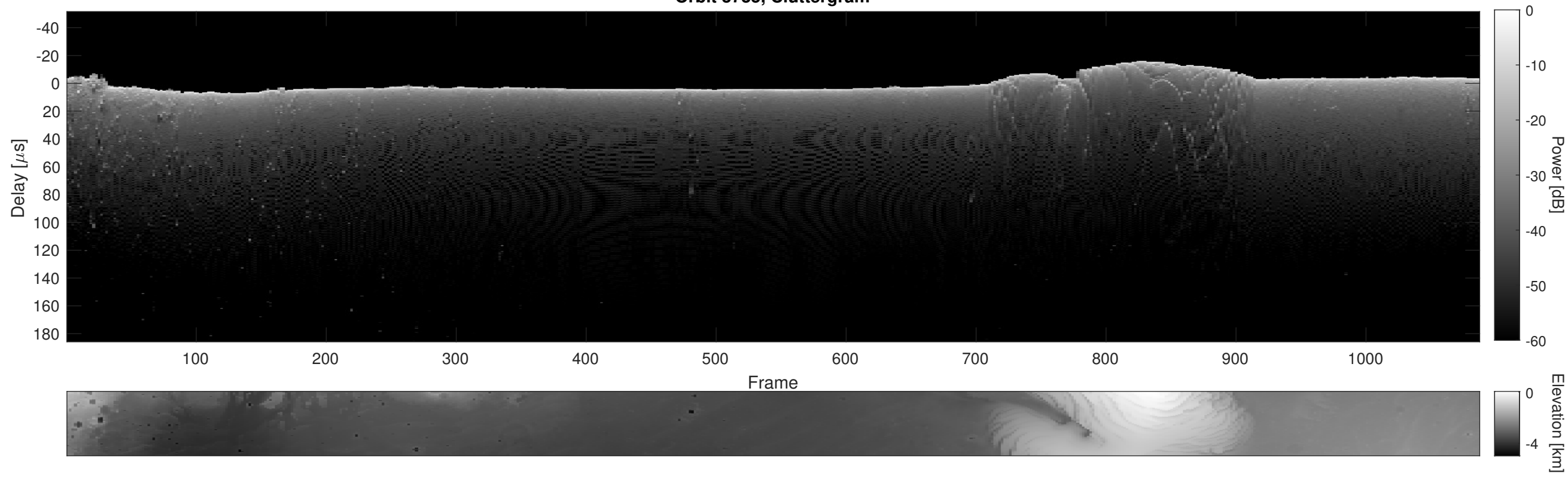
Orbit 3735, Cluttergram
