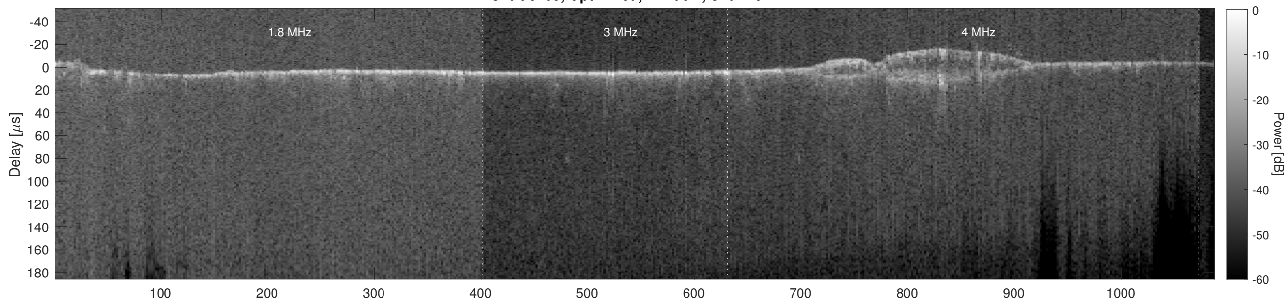
Orbit 3735, Cluttergram
