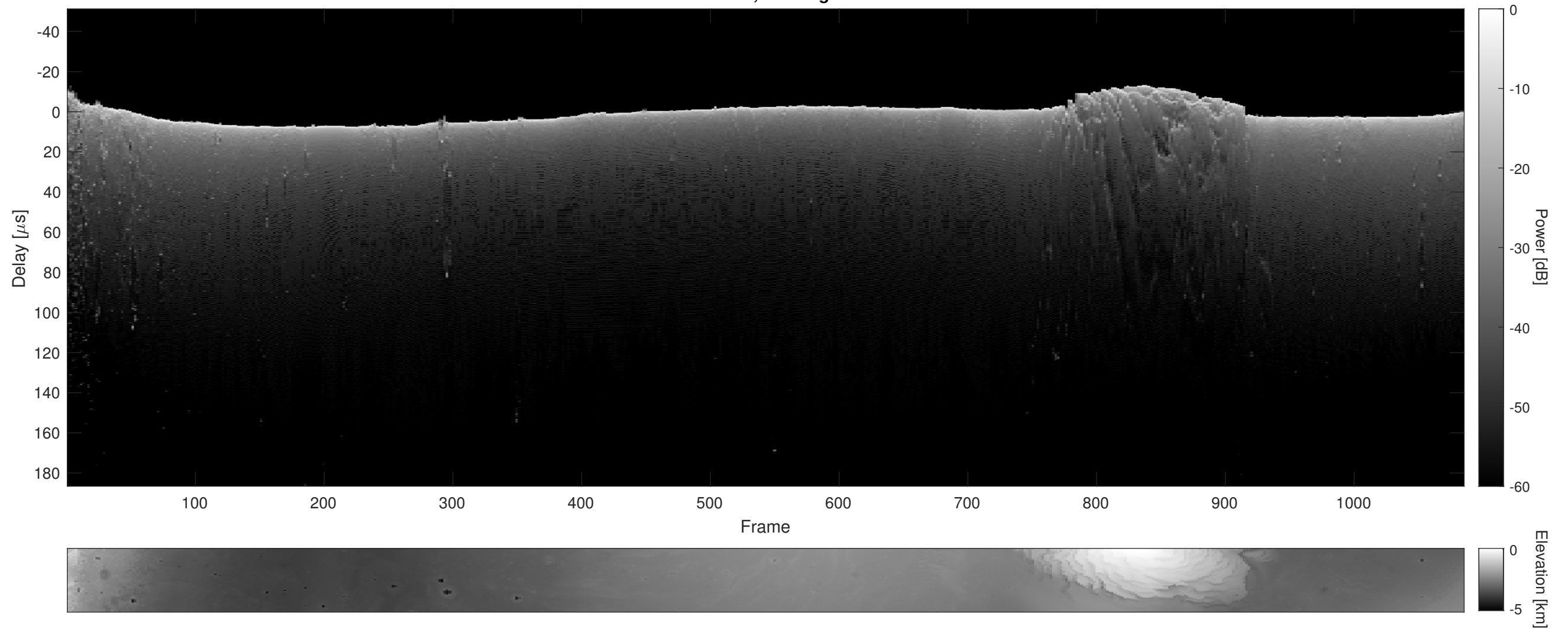
Orbit 3737, Cluttergram
