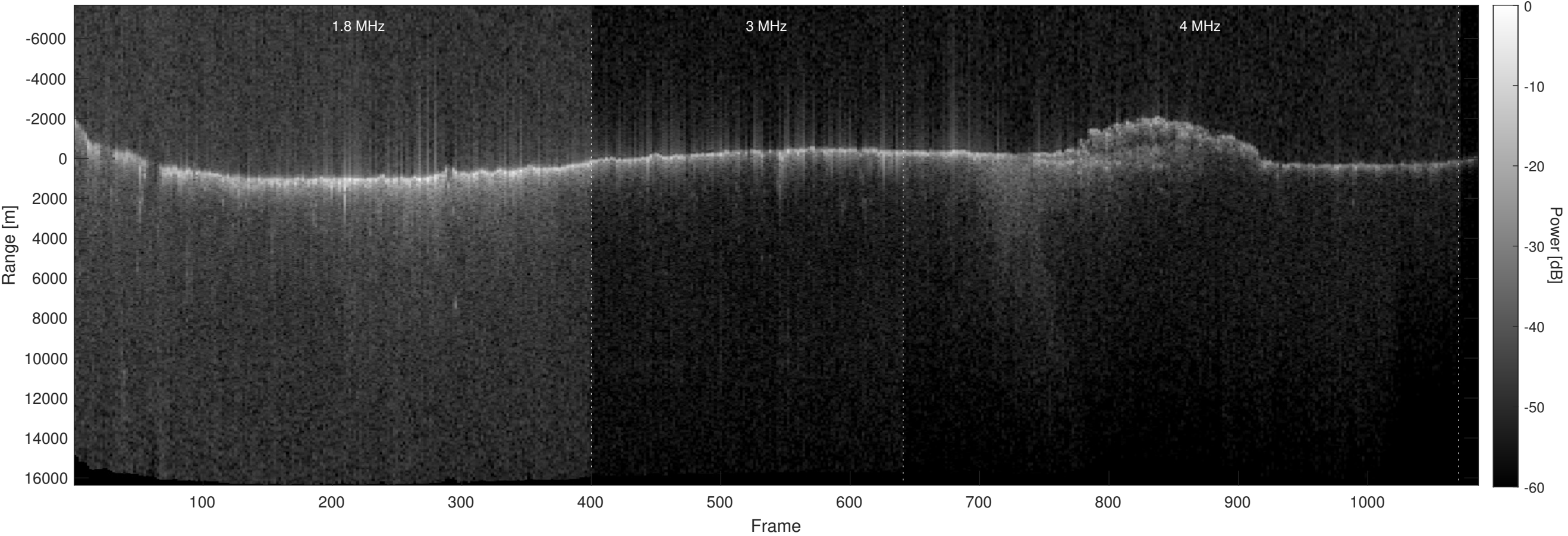
Orbit 3737, Optimized, No Window, Depth-Corrected, Channel 2
