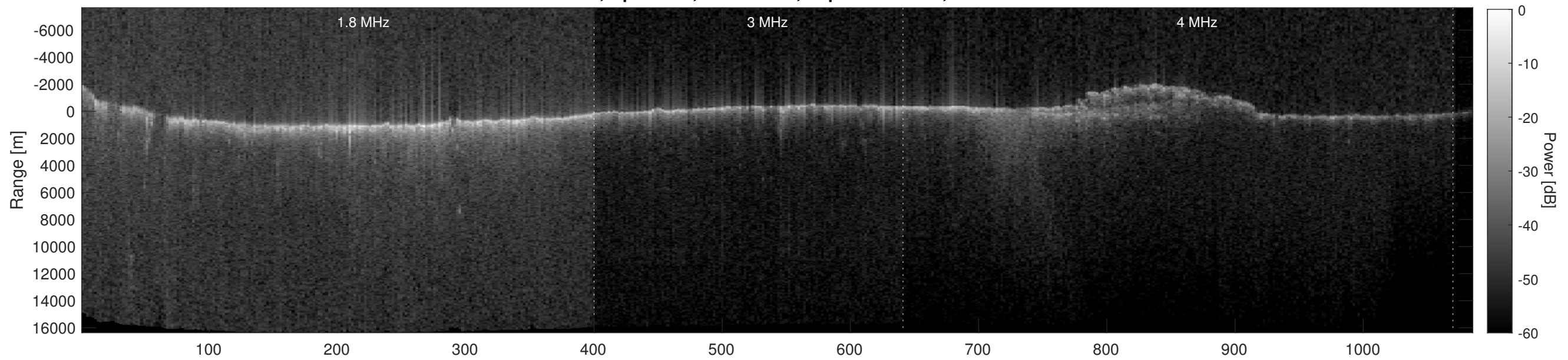
Orbit 3737, Depth-Corrected Cluttergram
