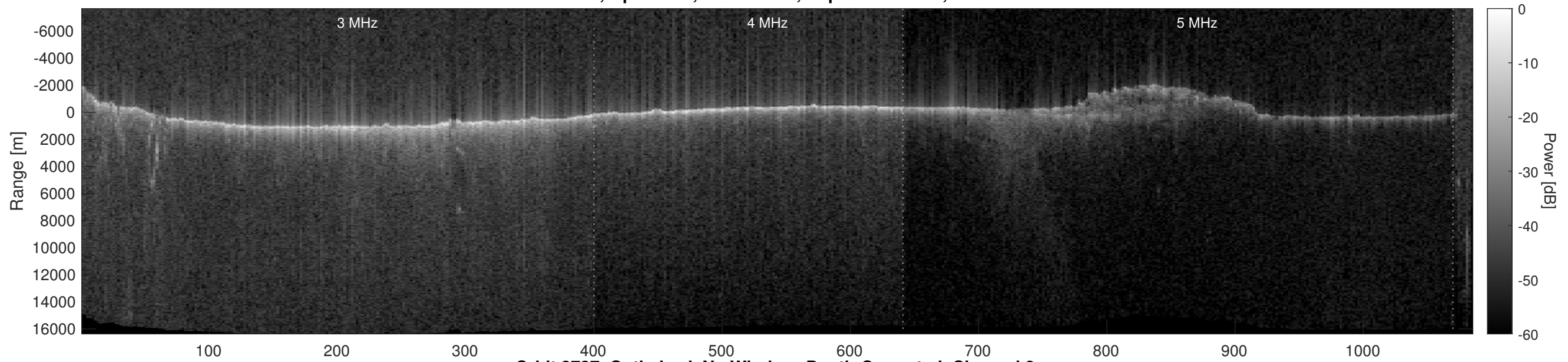
Orbit 3737, Optimized, No Window, Depth-Corrected, Channel 2
