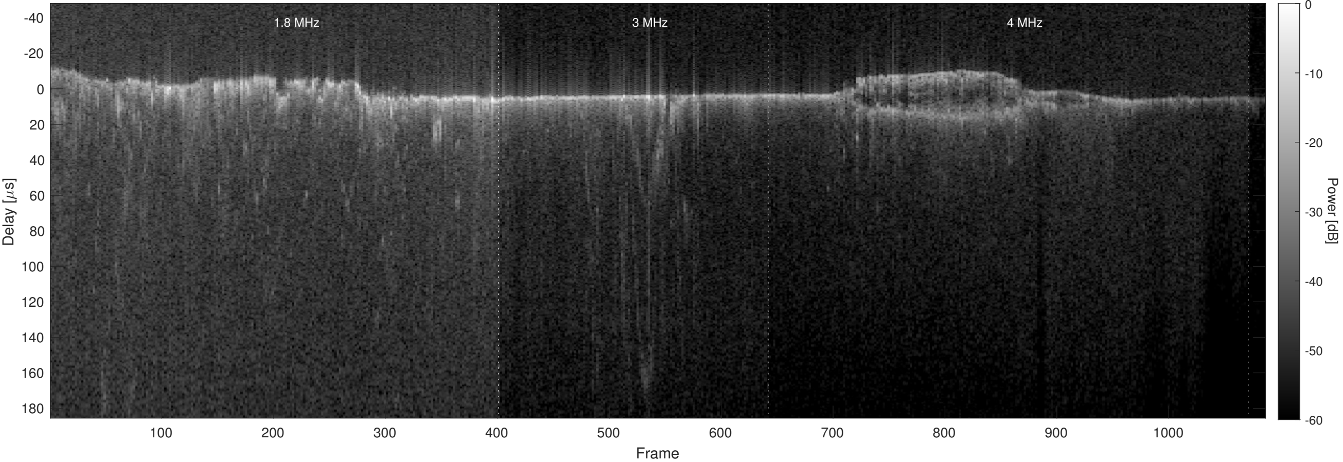
Orbit 3738, Optimized, No Window, Channel 2
