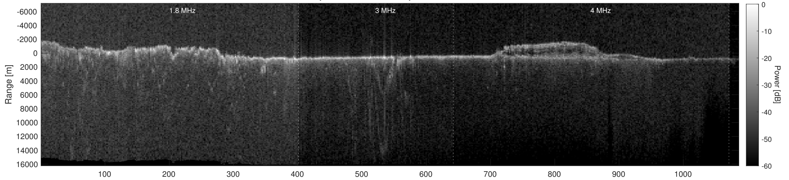
Orbit 3738, Depth-Corrected Cluttergram
