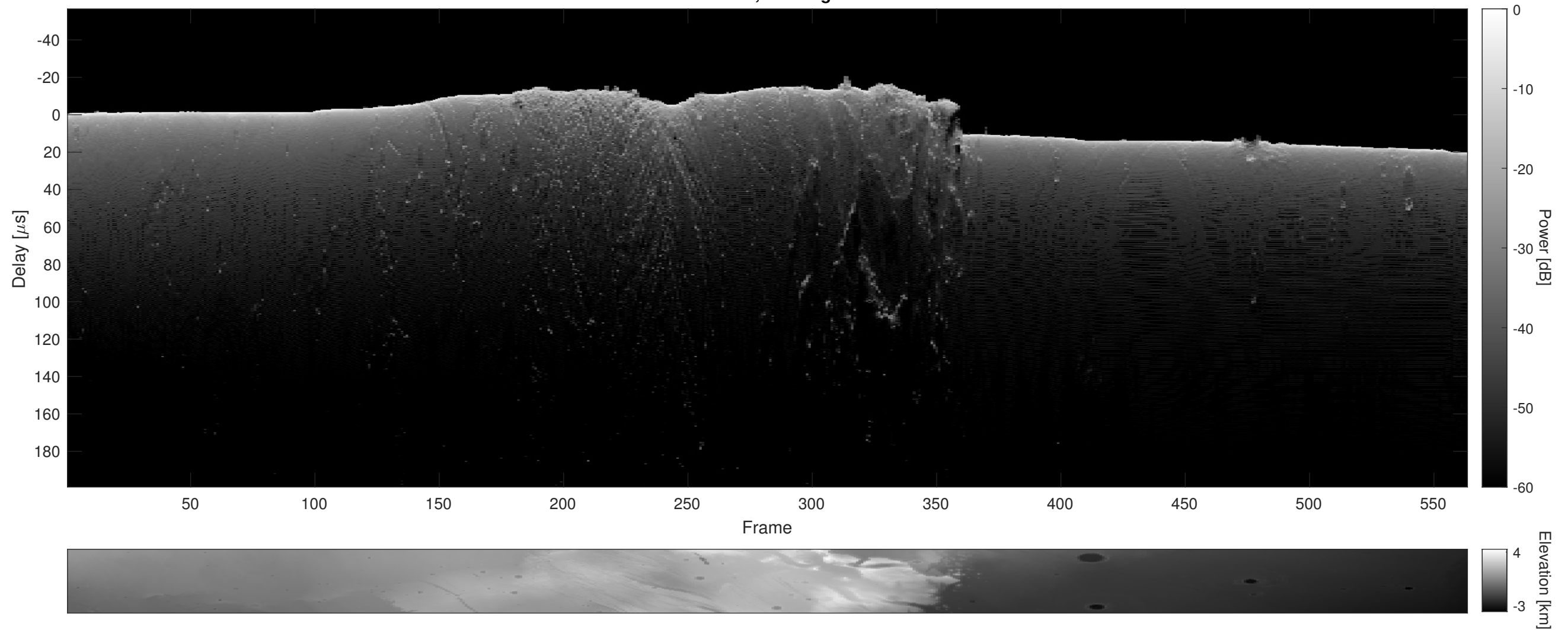
Orbit 3739, Cluttergram
