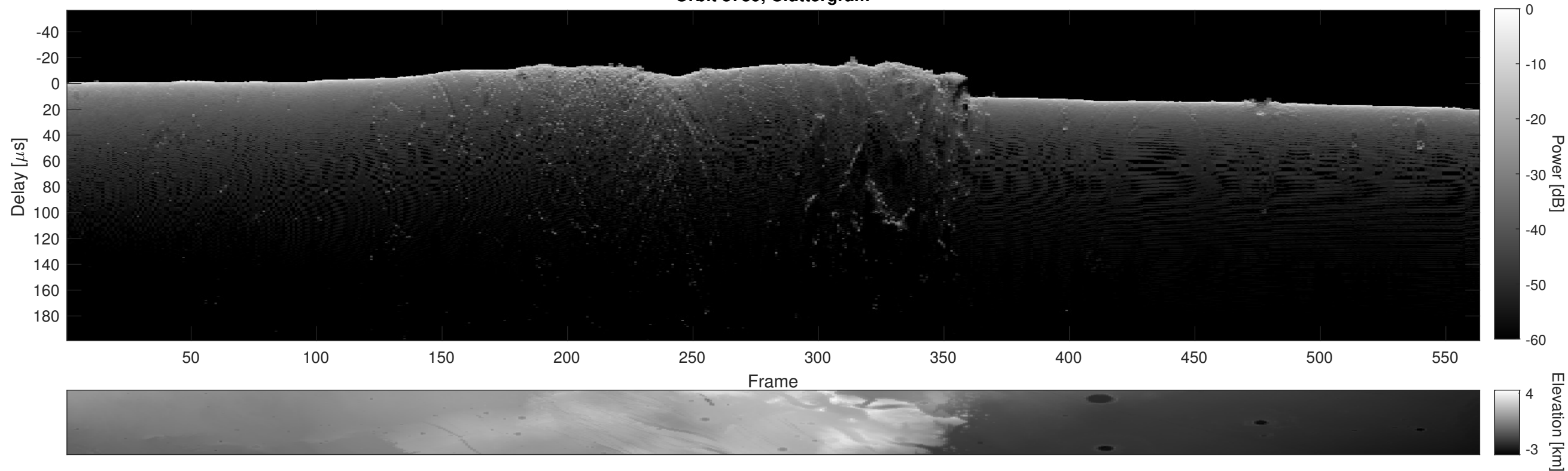
Orbit 3739, Cluttergram
