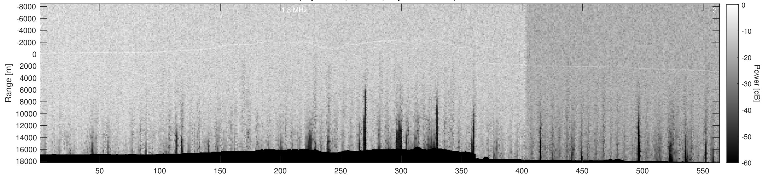
Orbit 3739, Depth-Corrected Cluttergram
