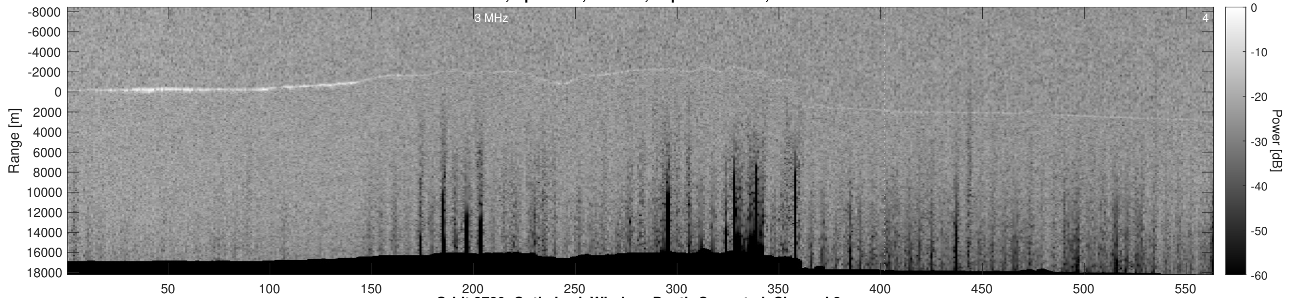
Orbit 3739, Optimized, Window, Depth-Corrected, Channel 2
