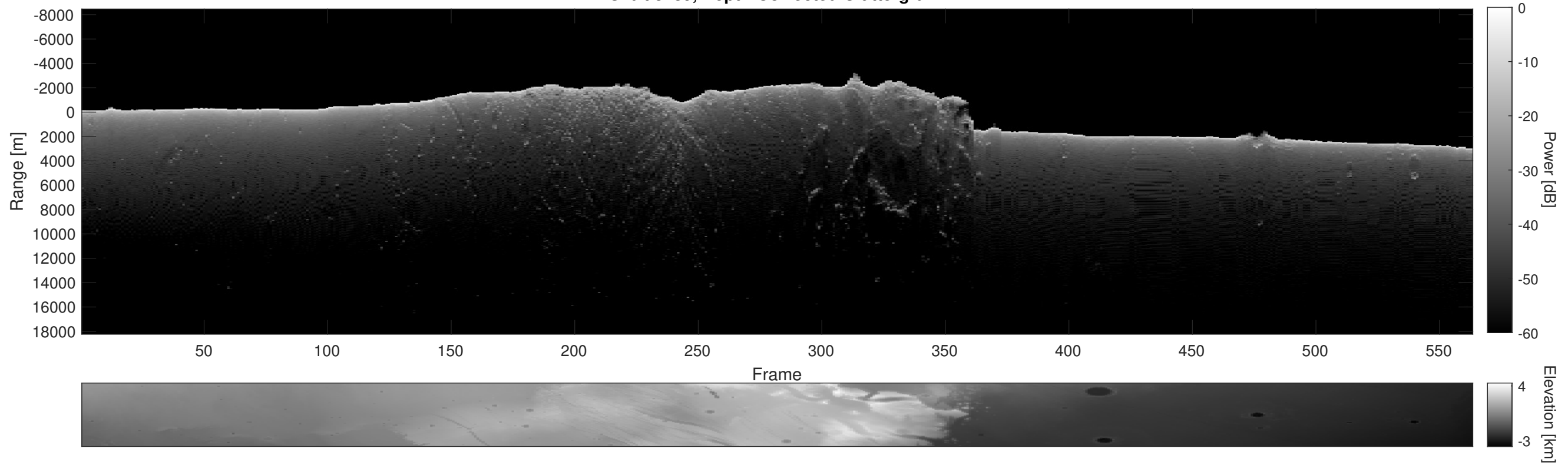
Orbit 3739, Depth-Corrected Cluttergram
