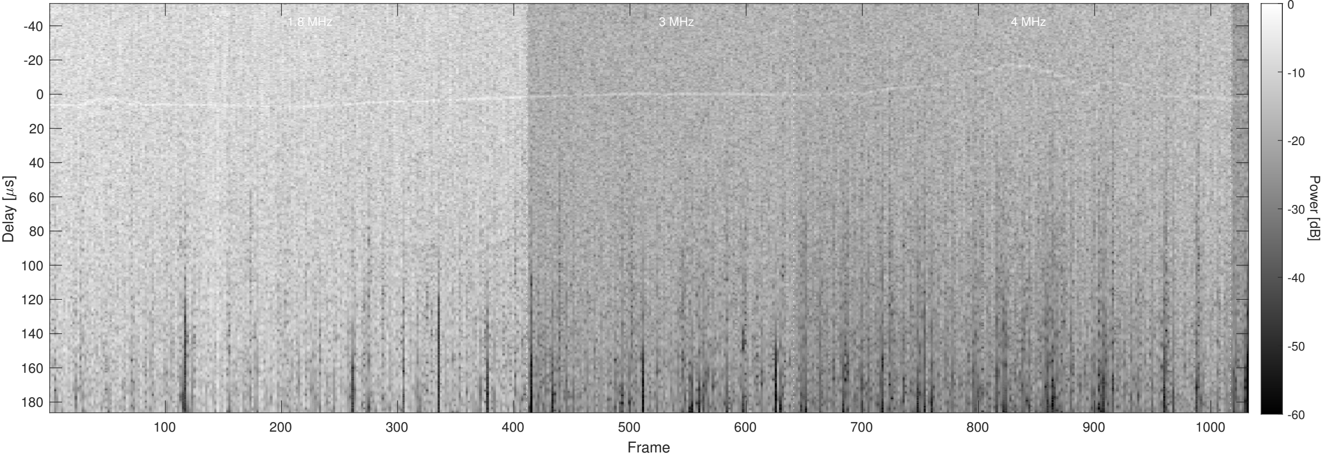
Orbit 3740, Optimized, No Window, Channel 2
