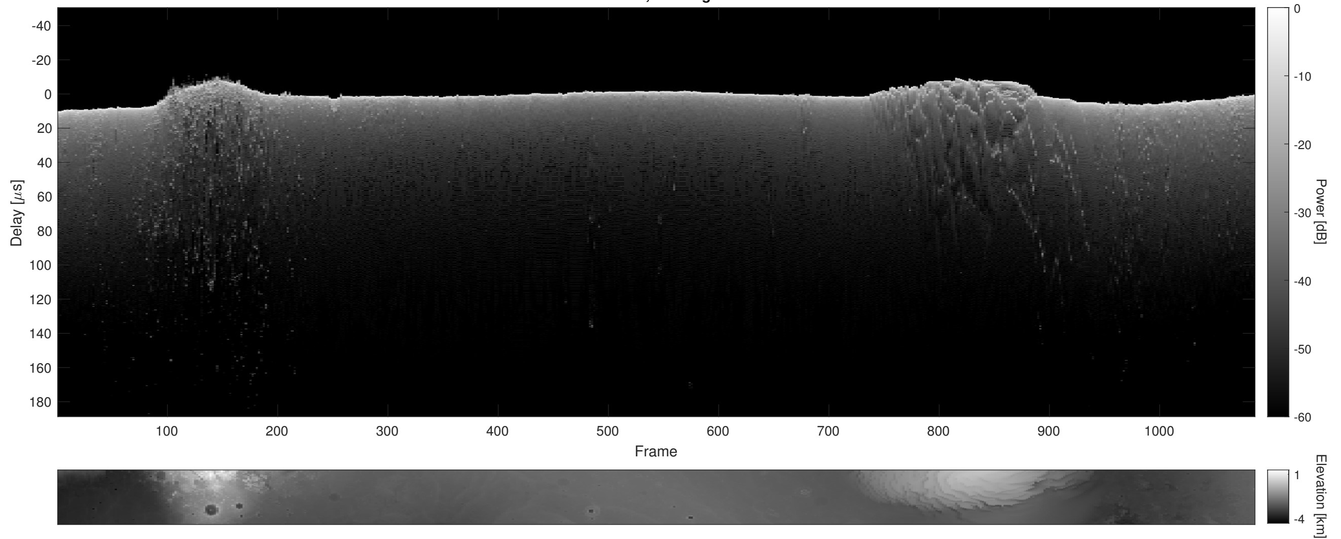
Orbit 3741, Cluttergram
