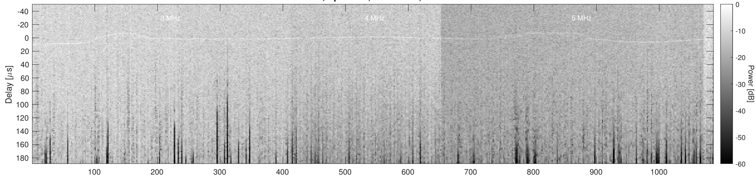
Orbit 3741, Optimized, No Window, Channel 2
