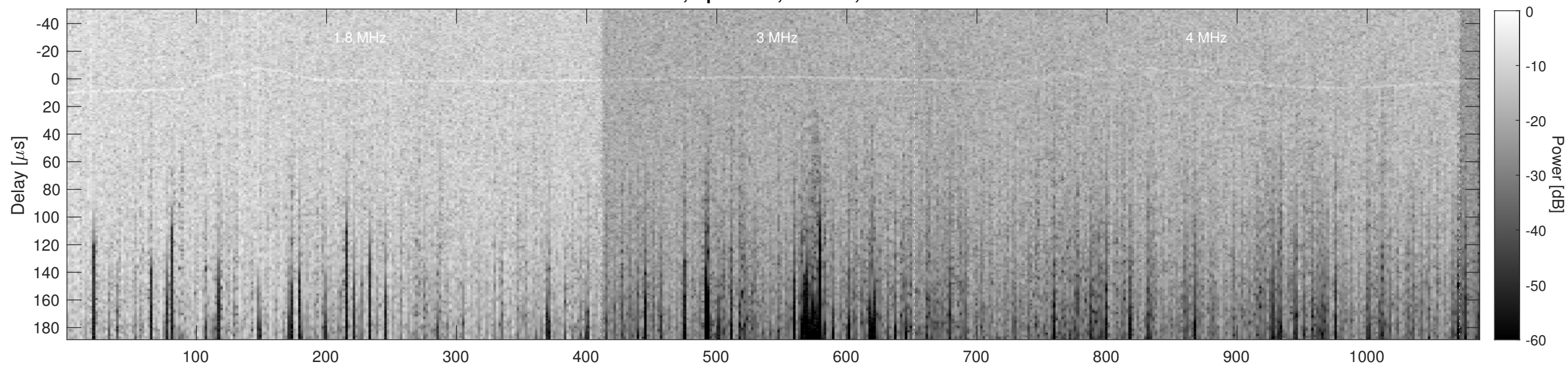
Orbit 3741, Cluttergram
