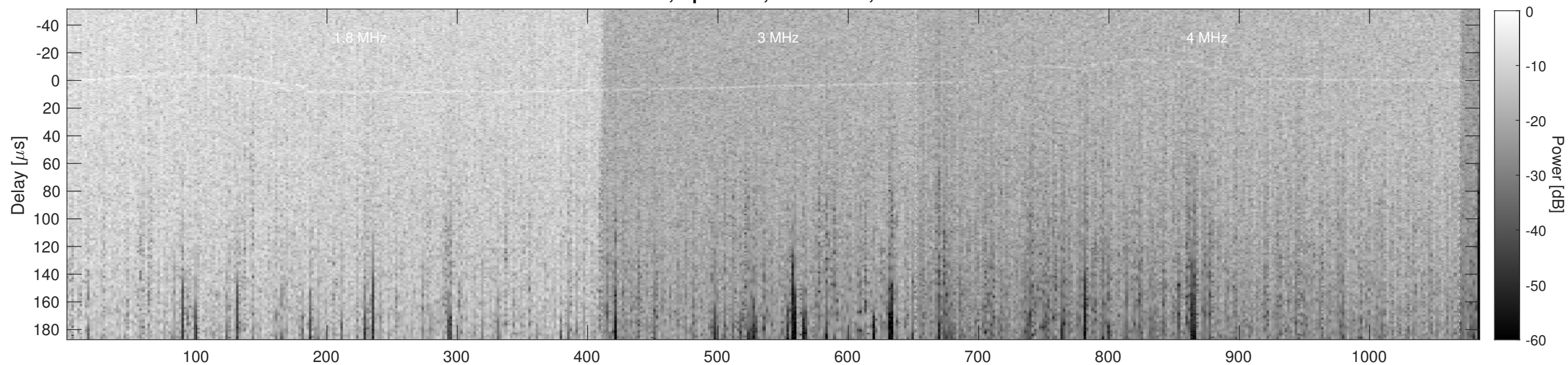
Orbit 3742, Cluttergram
