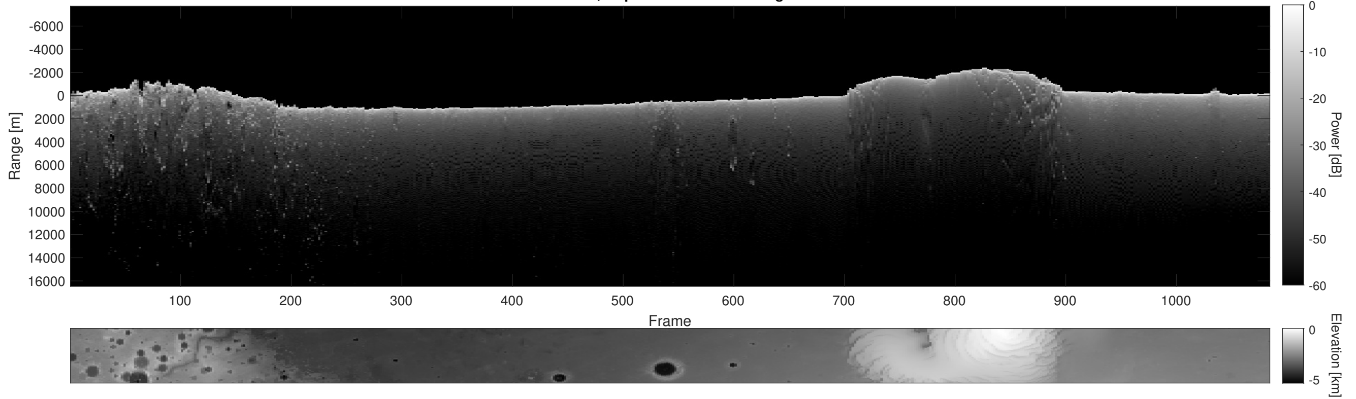
Orbit 3742, Depth-Corrected Cluttergram
