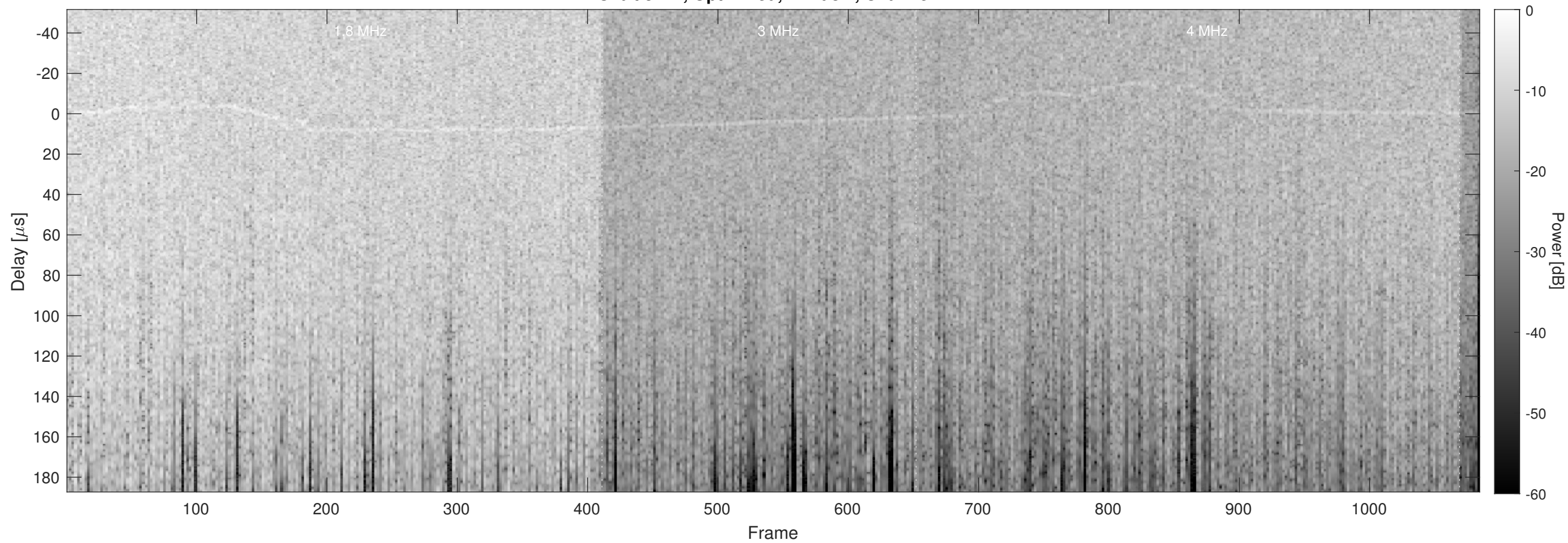
Orbit 3742, Optimized, Window, Channel 2
