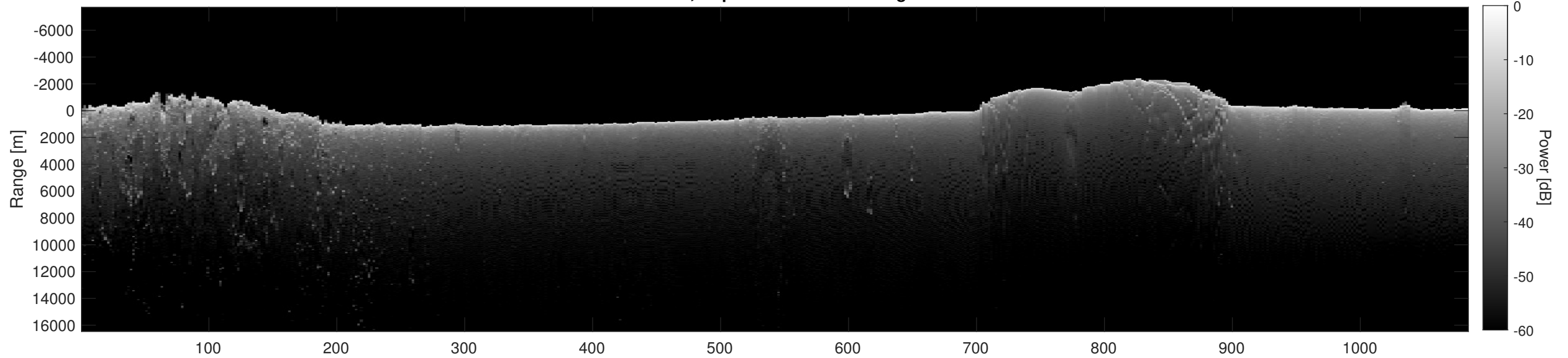
Orbit 3742, Depth-Corrected Cluttergram
