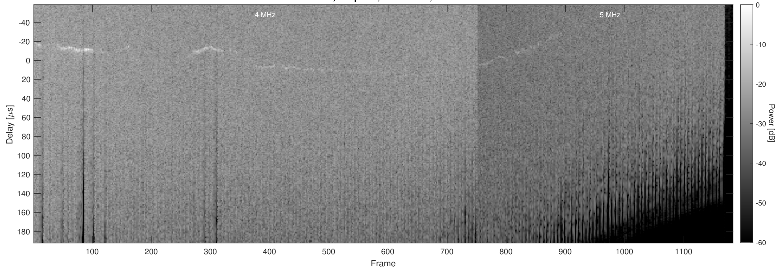
Orbit 3745, Chapman, No Window, Channel 2
