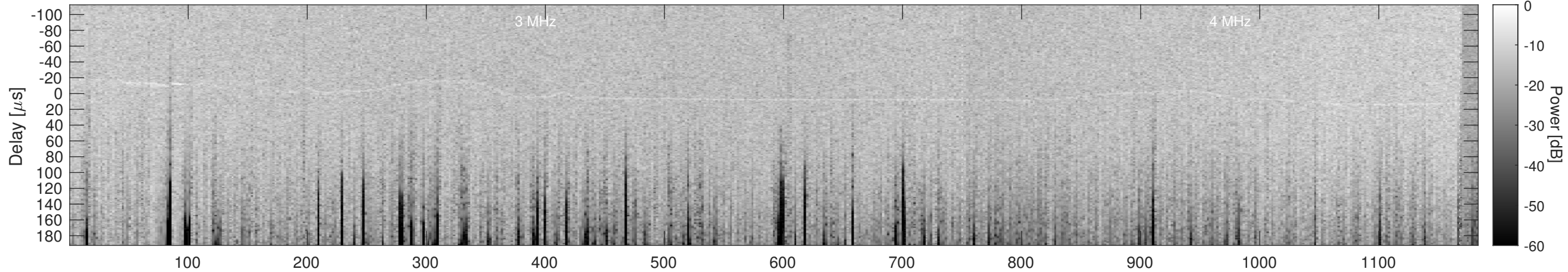
Orbit 3745, Cluttergram
