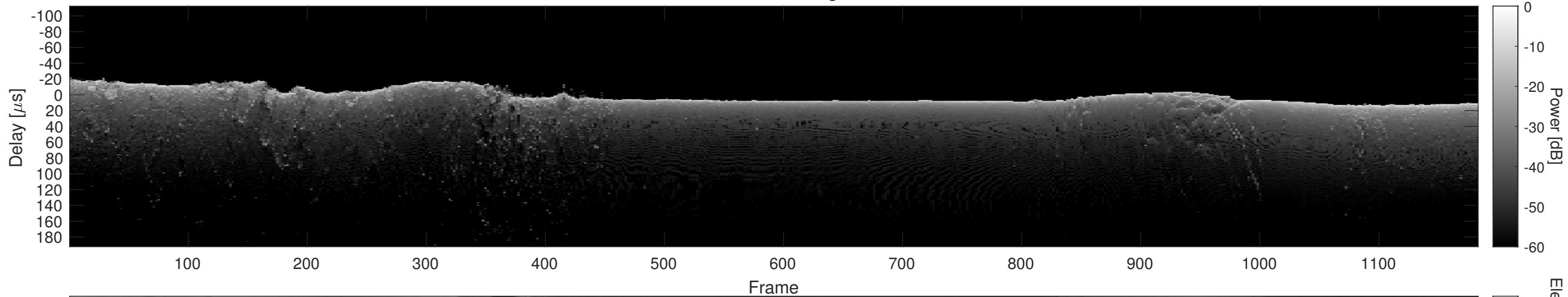
Orbit 3745, Cluttergram
