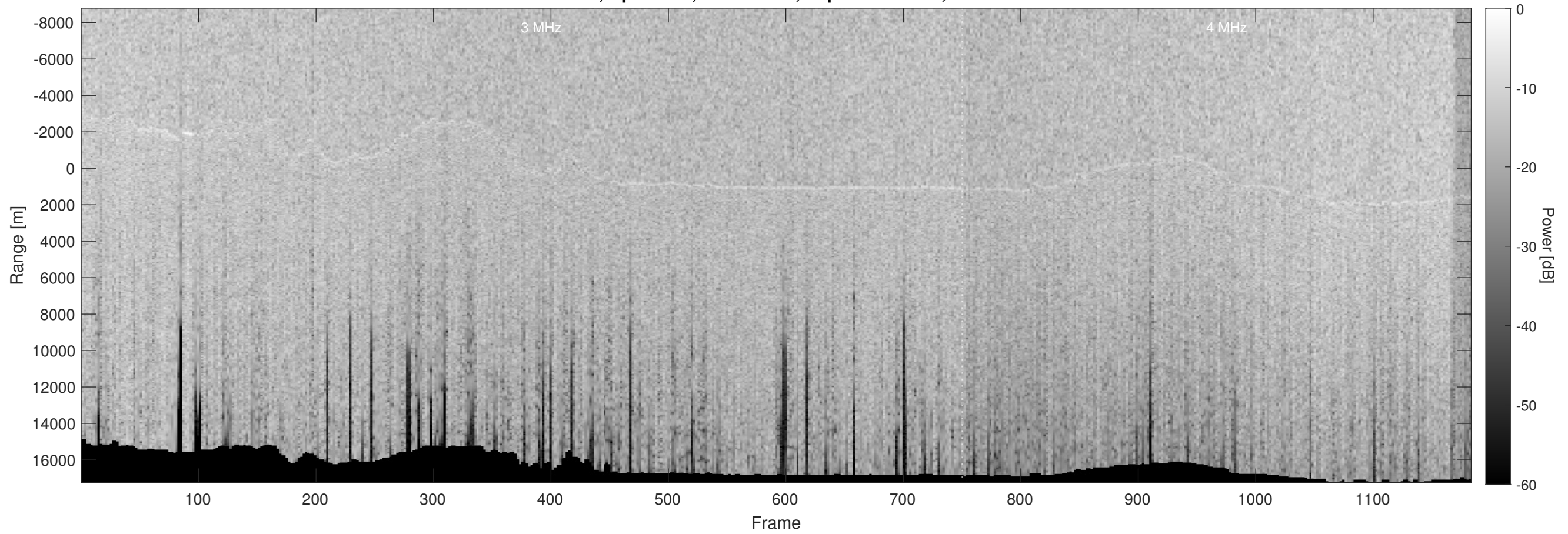
Orbit 3745, Optimized, No Window, Depth-Corrected, Channel 2
