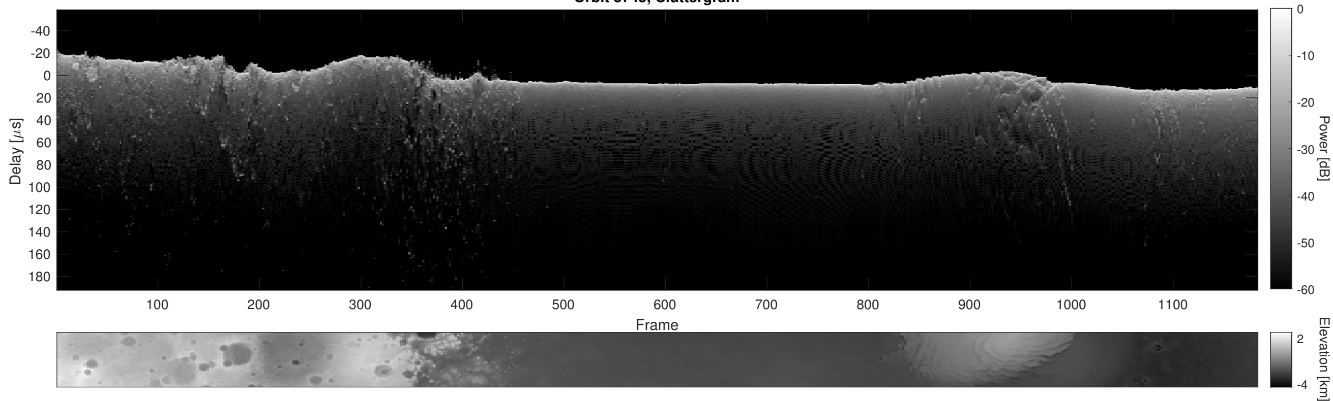
Orbit 3745, Cluttergram
