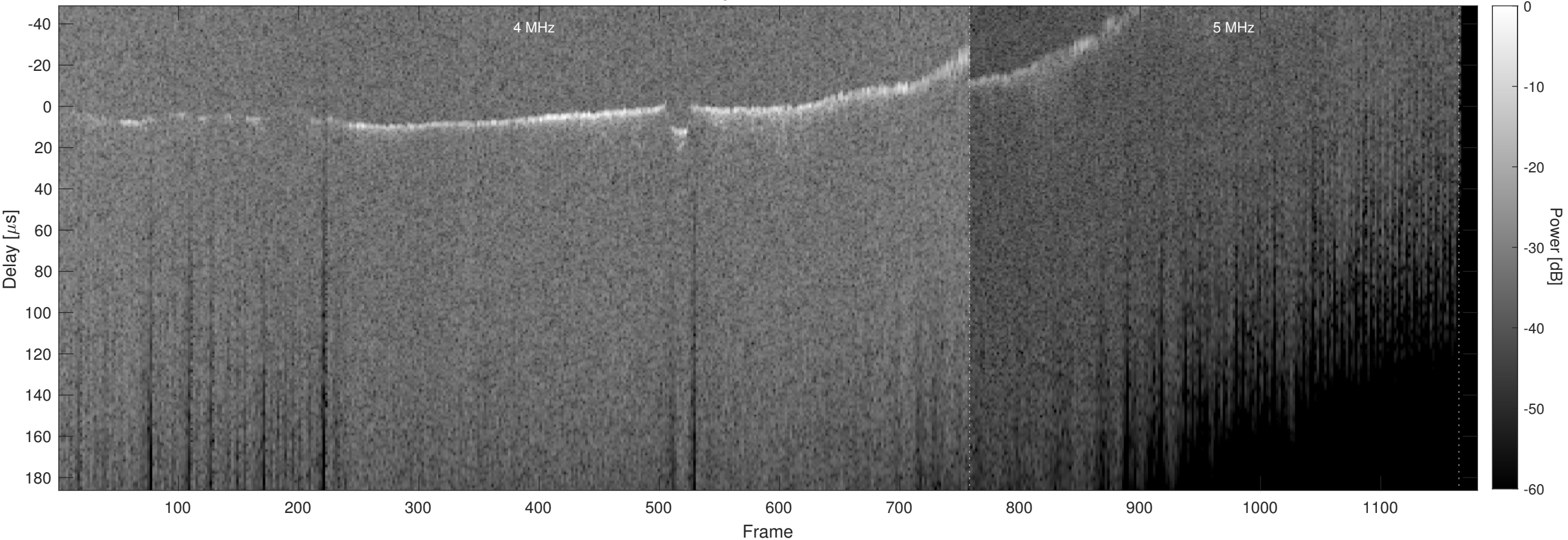
Orbit 3747, Chapman, Window, Channel 2
