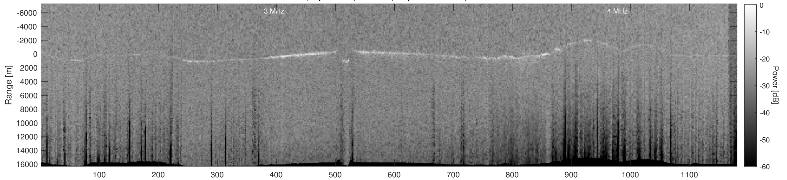
Orbit 3747, Depth-Corrected Cluttergram
