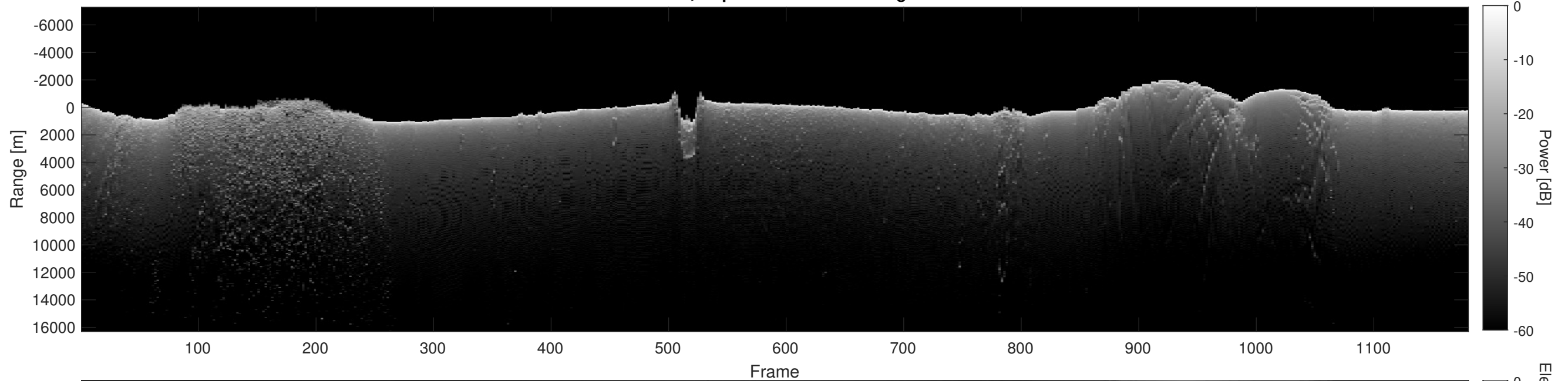
Orbit 3747, Depth-Corrected Cluttergram
