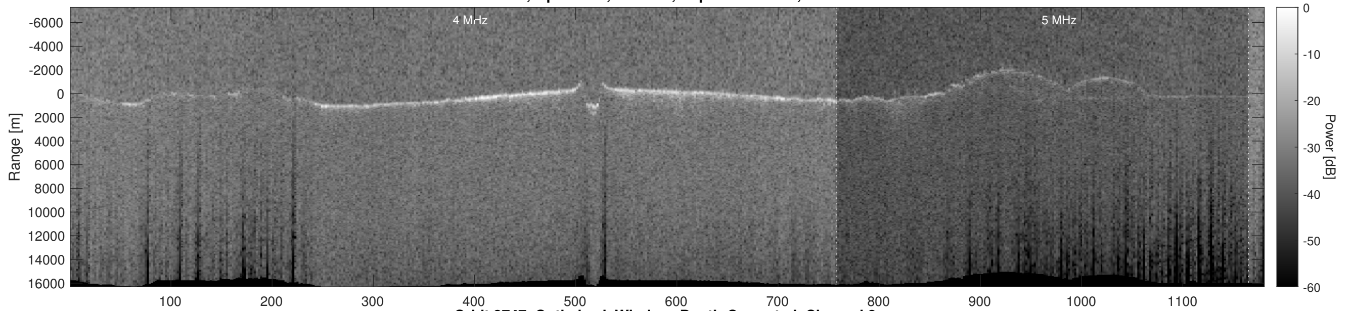
Orbit 3747, Optimized, Window, Depth-Corrected, Channel 2
