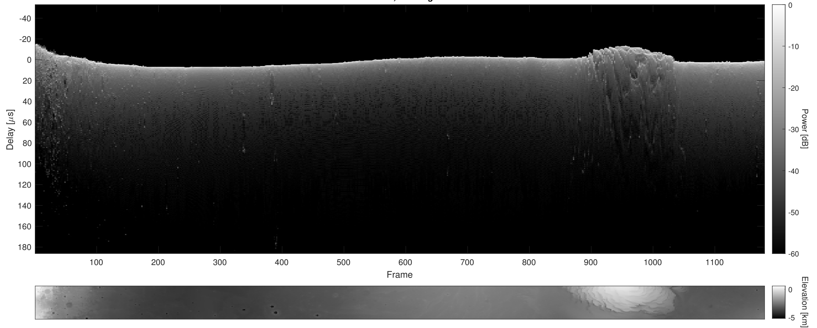
Orbit 3748, Cluttergram
