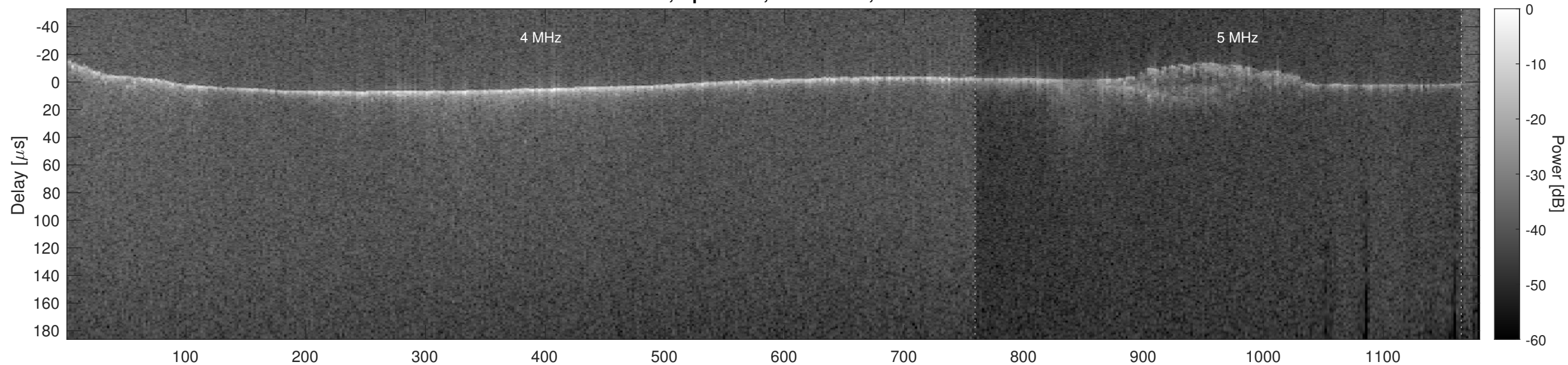
Orbit 3748, Optimized, No Window, Channel 2
