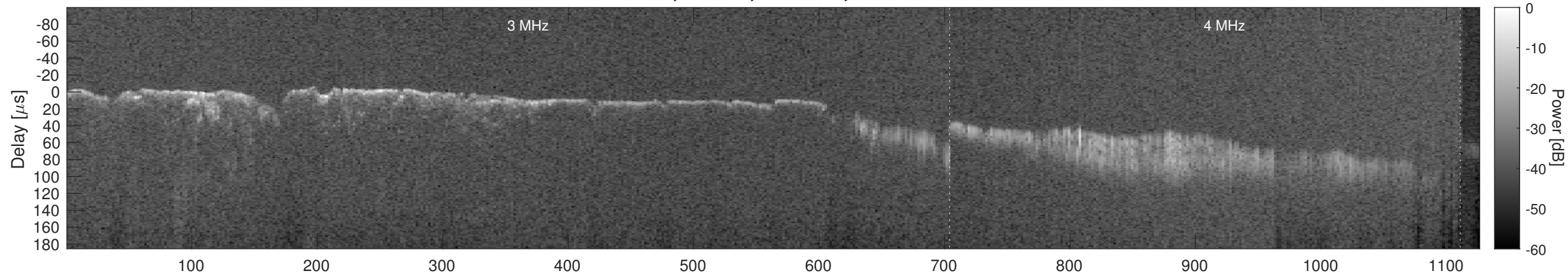
Orbit 3749, Window, Channel 2, Chapman
