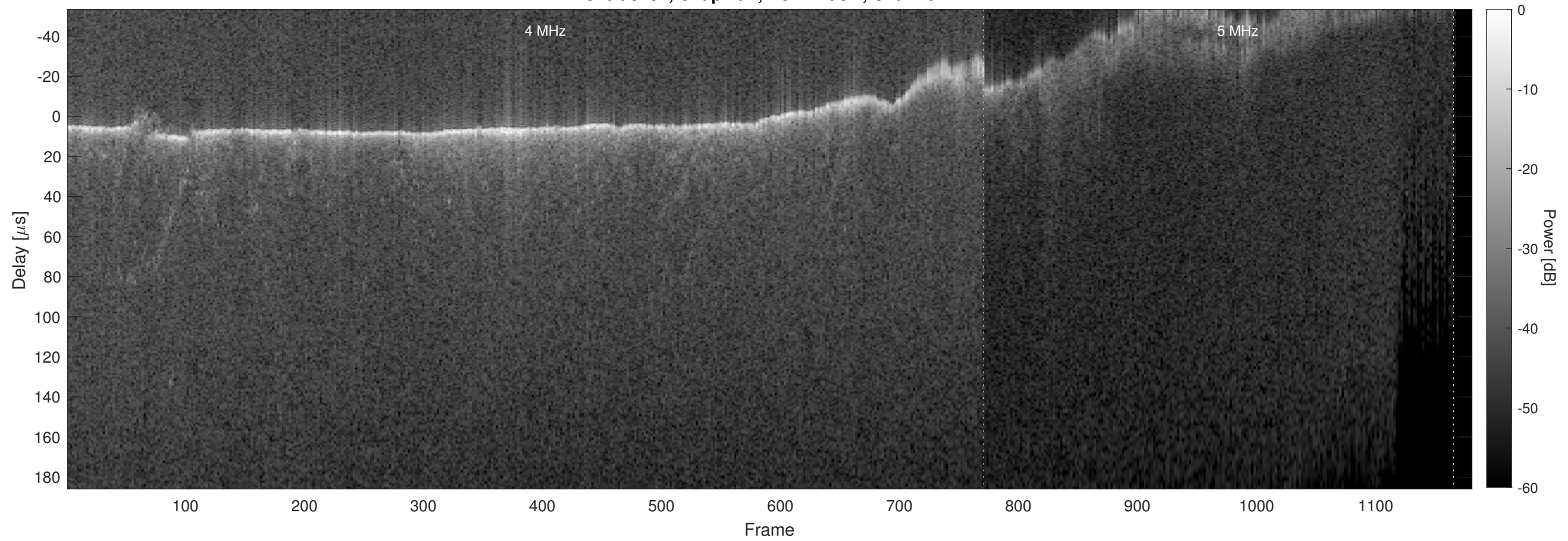
Orbit 3751, Chapman, No Window, Channel 2
