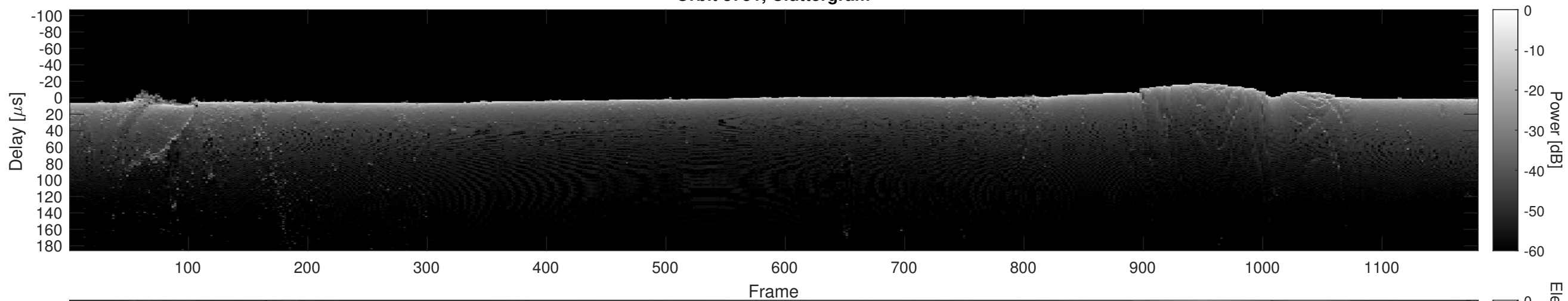
Orbit 3751, Cluttergram
