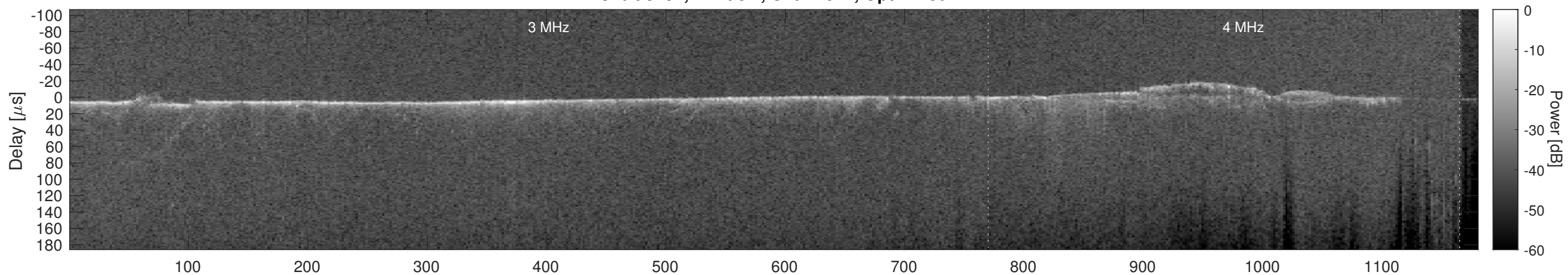
Orbit 3751, Cluttergram
