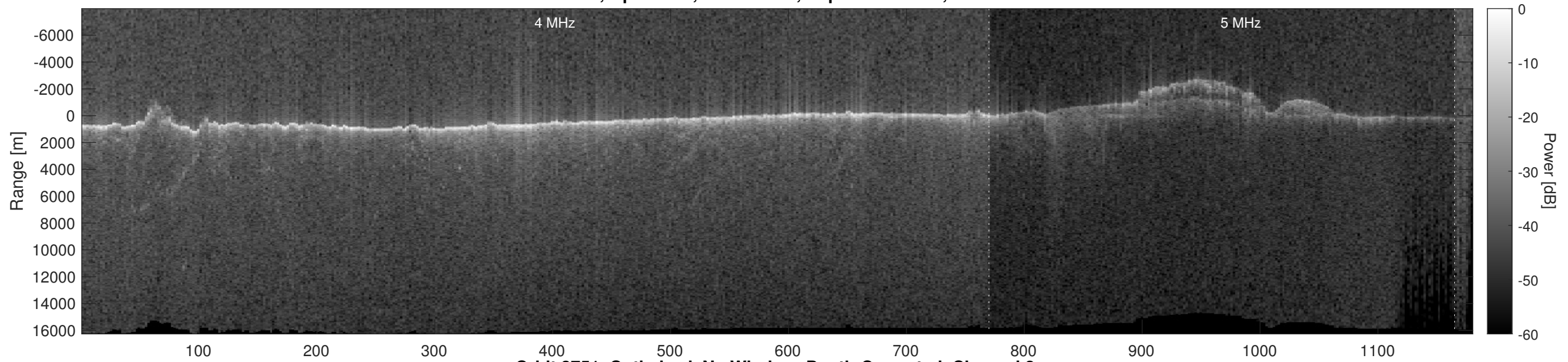
Orbit 3751, Optimized, No Window, Depth-Corrected, Channel 2
