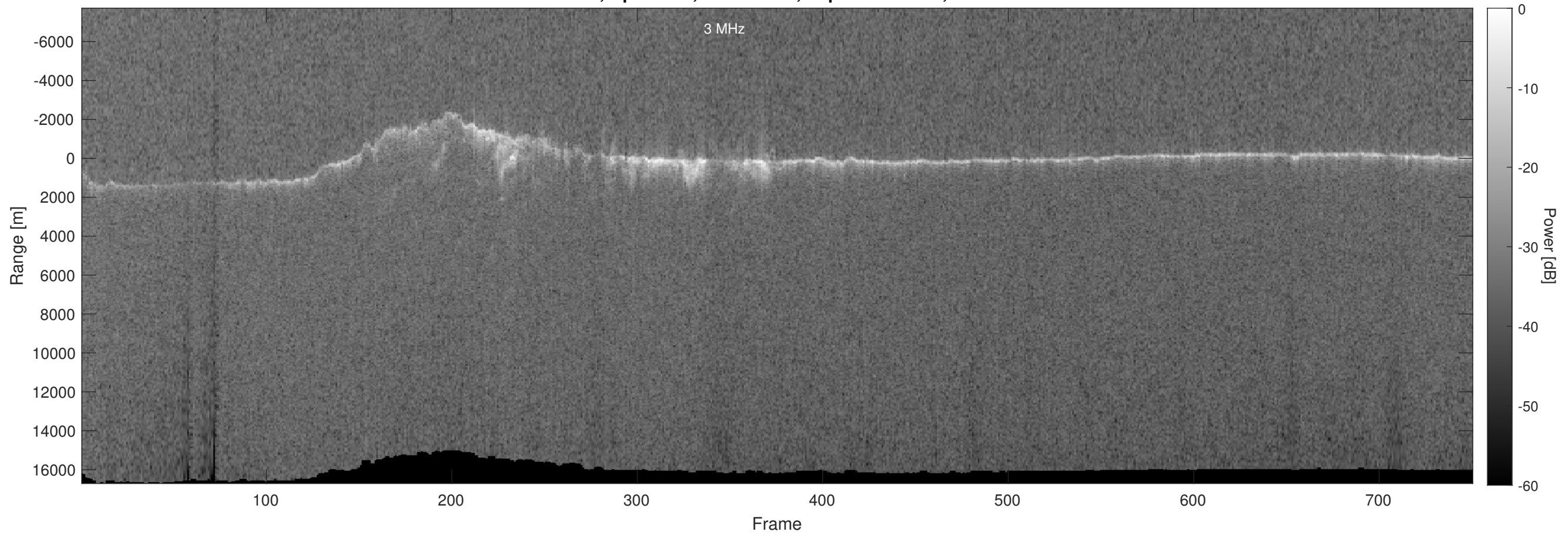
Orbit 3752, Optimized, No Window, Depth-Corrected, Channel 2
