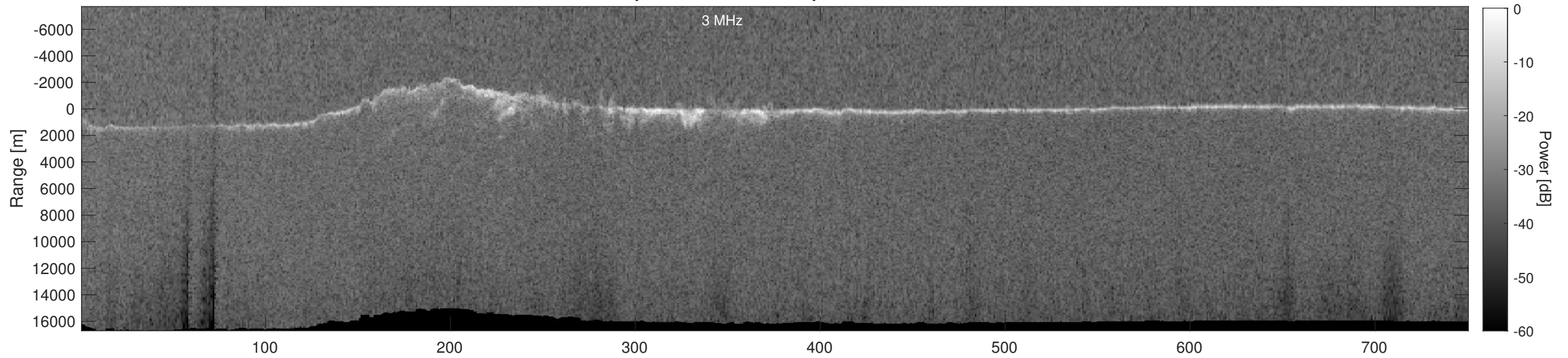
Orbit 3752, Depth-Corrected Cluttergram
