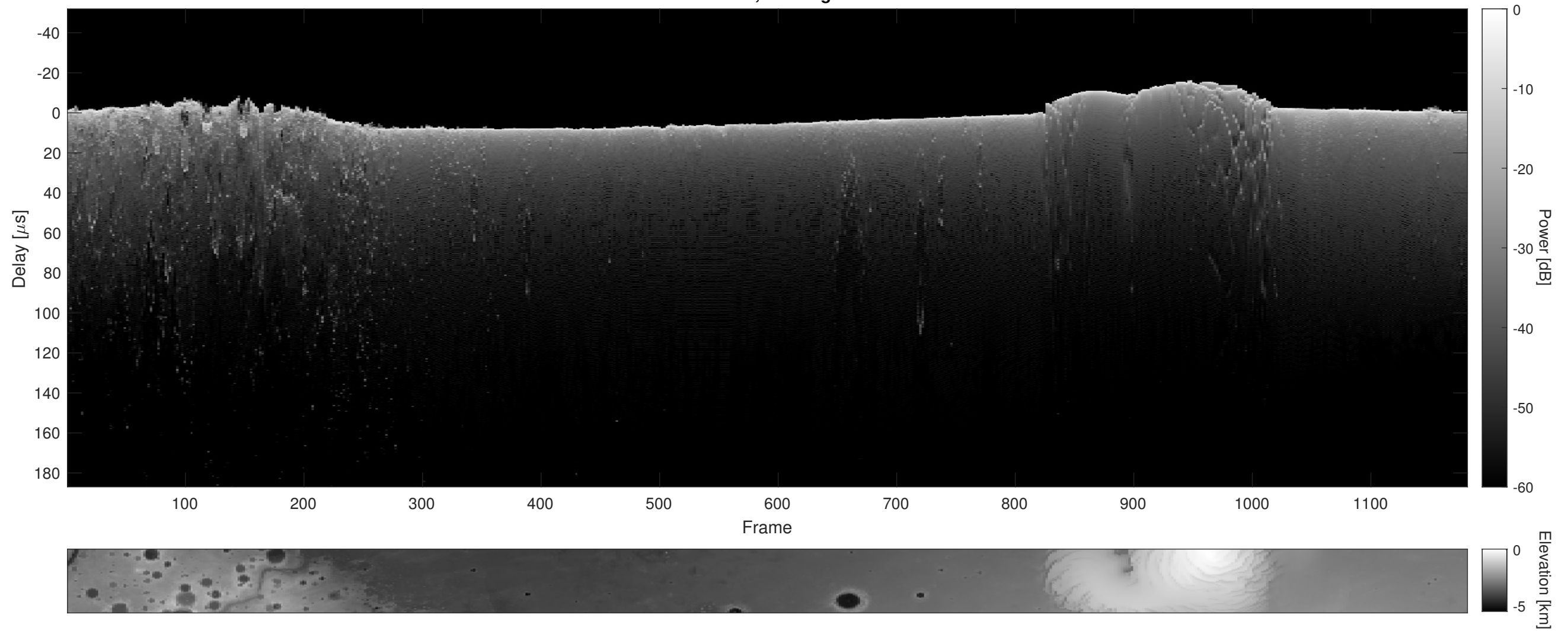
Orbit 3753, Cluttergram
