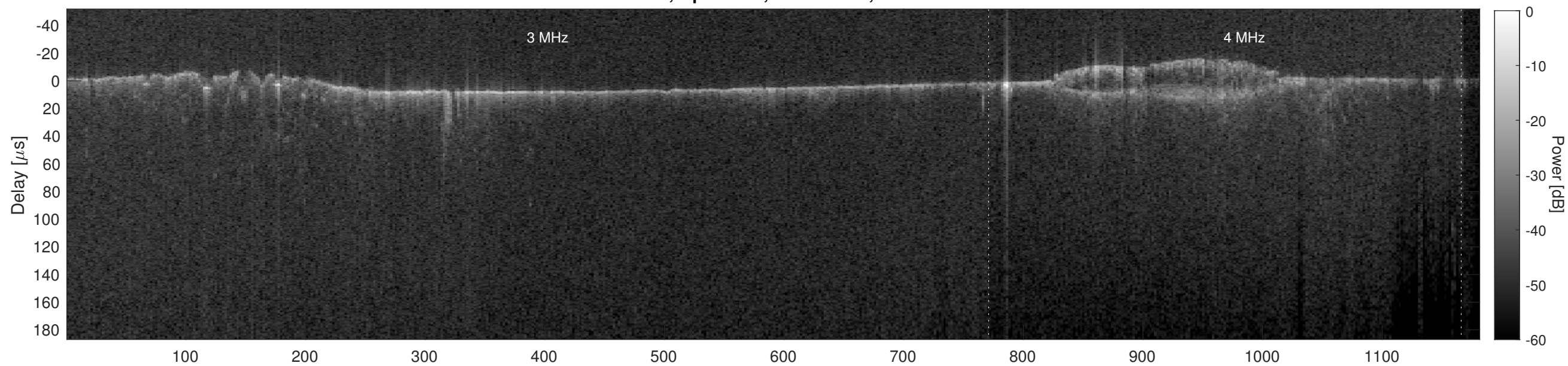
Orbit 3753, Cluttergram
