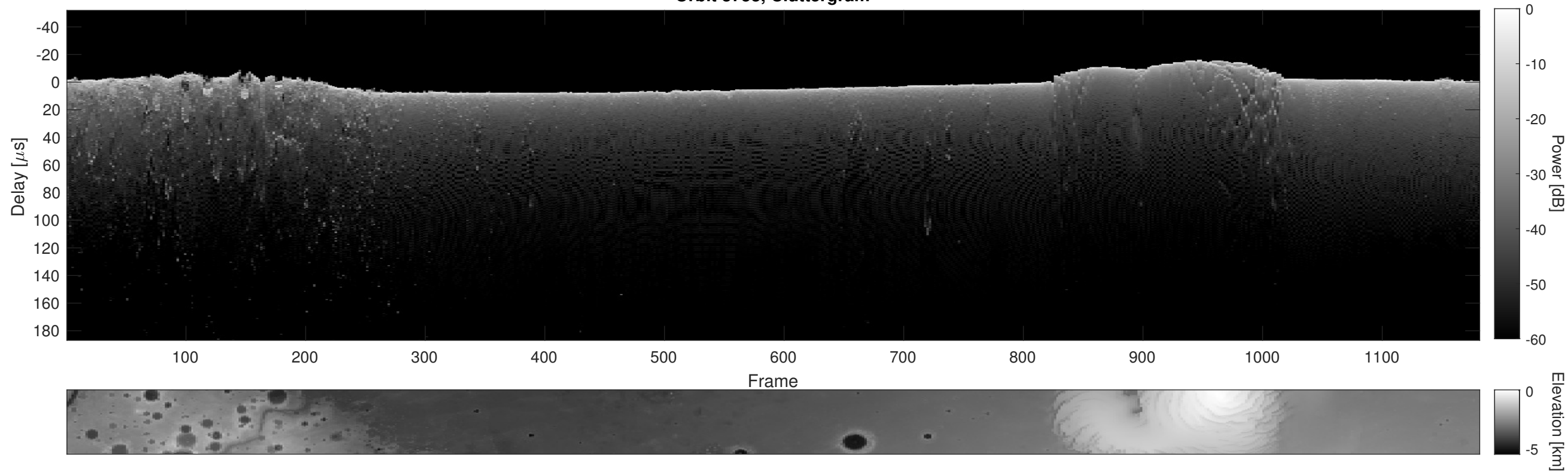
Orbit 3753, Cluttergram
