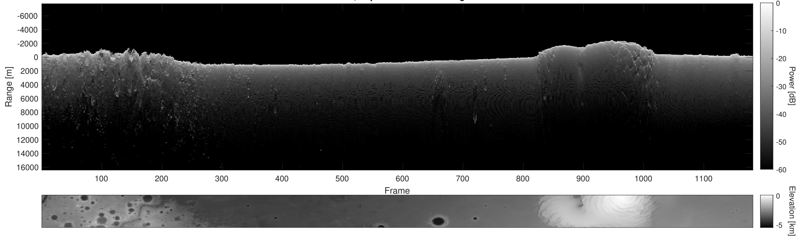
Orbit 3753, Depth-Corrected Cluttergram
