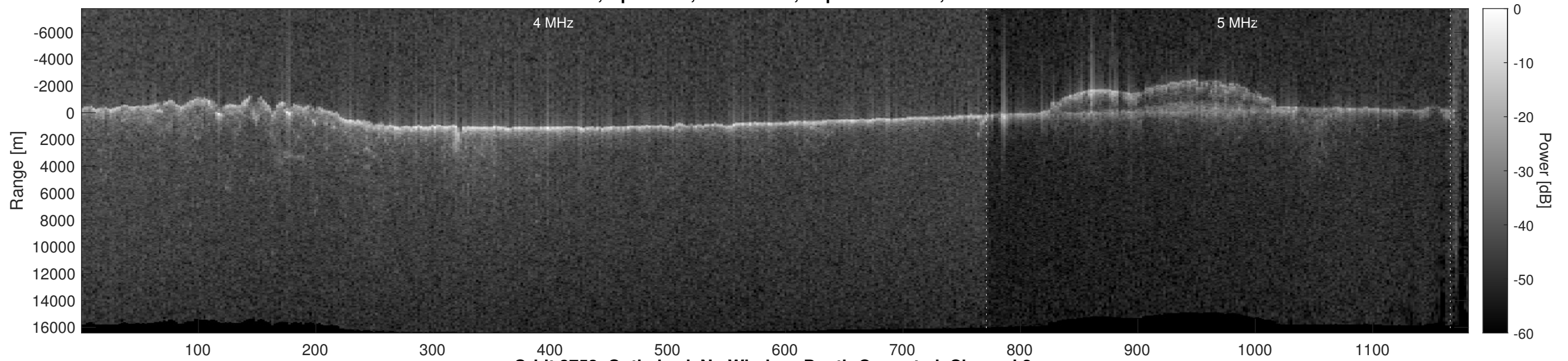
Orbit 3753, Optimized, No Window, Depth-Corrected, Channel 2
