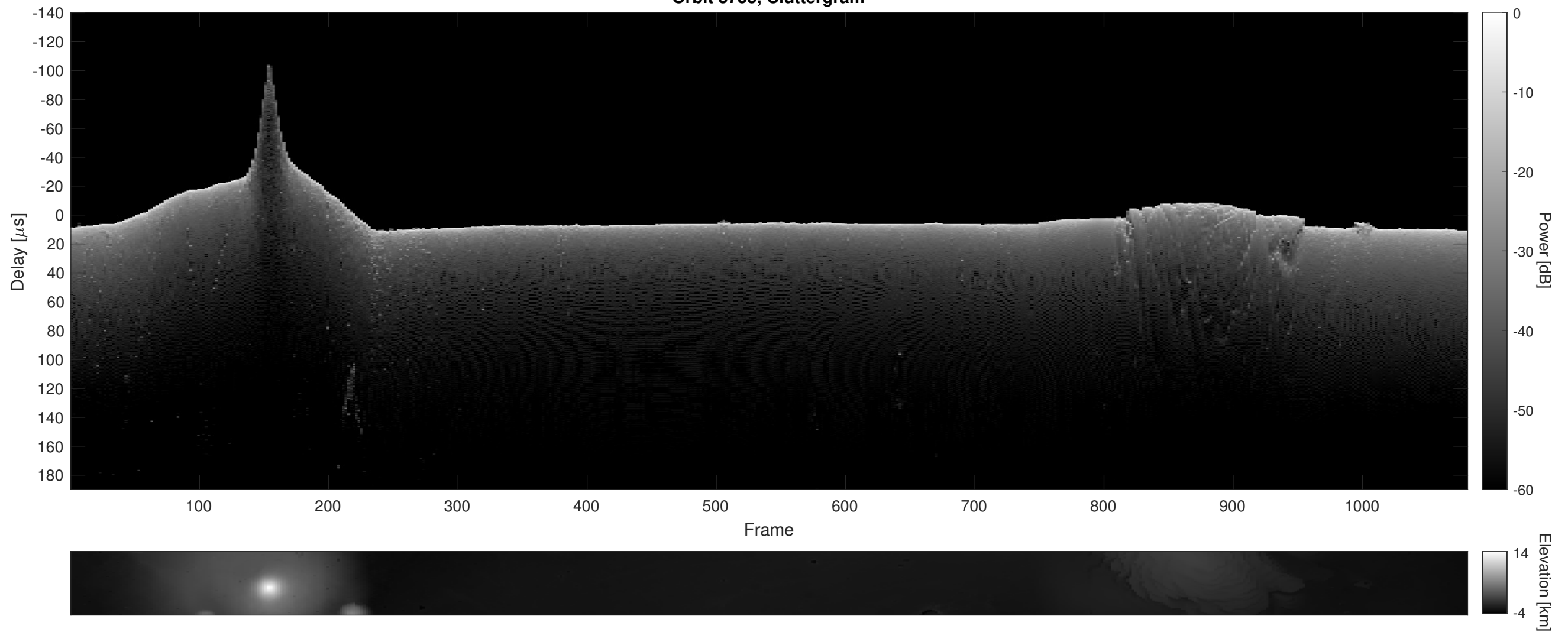
Orbit 3755, Cluttergram
