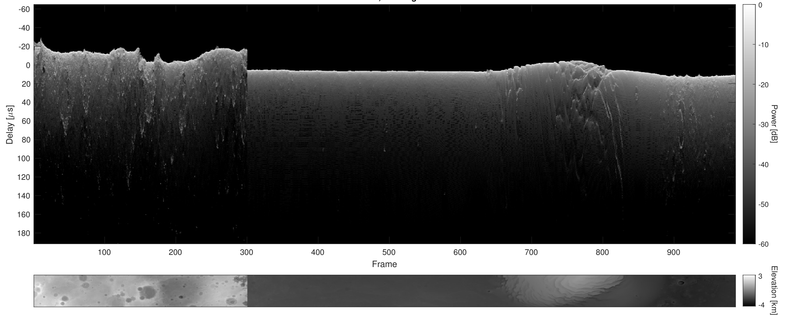
Orbit 3756, Cluttergram
