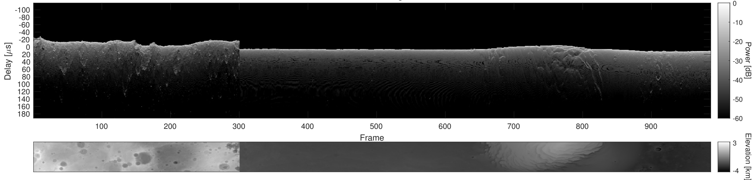
Orbit 3756, Cluttergram
