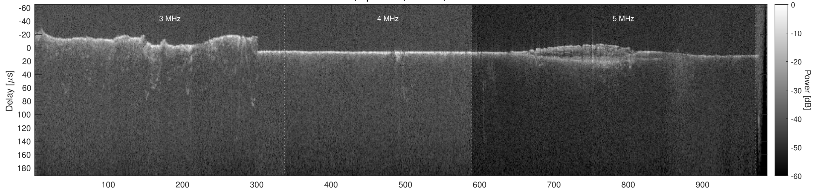
Orbit 3756, Optimized, Window, Channel 2
