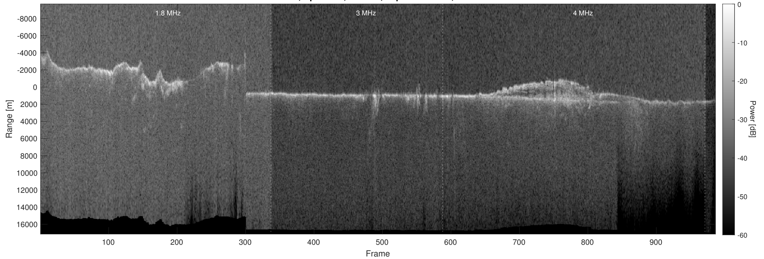
Orbit 3756, Optimized, Window, Depth-Corrected, Channel 2
