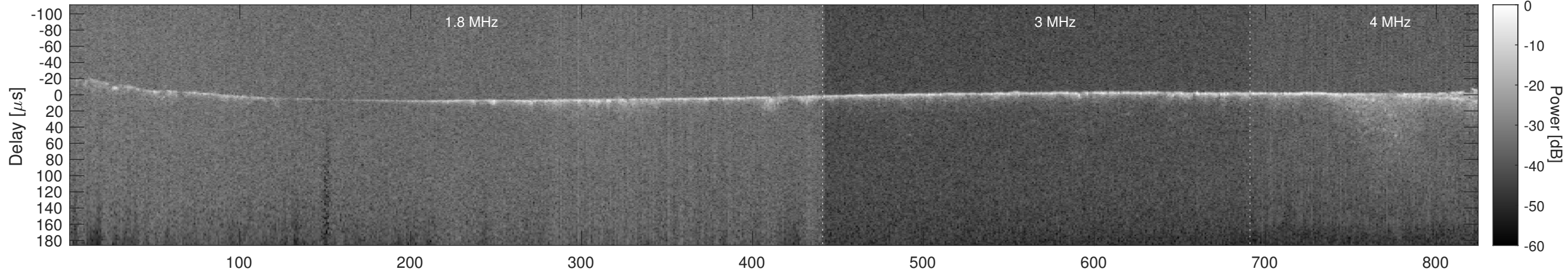
Orbit 3759, Cluttergram
