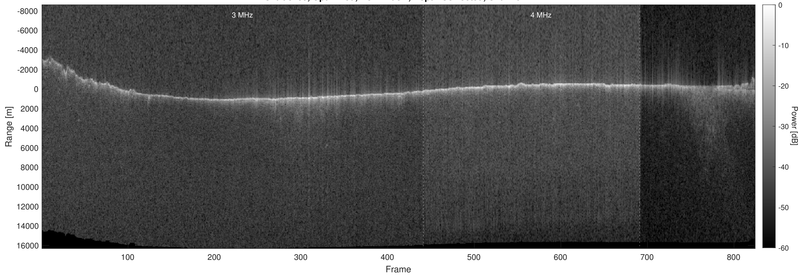
Orbit 3759, Optimized, No Window, Depth-Corrected, Channel 2
