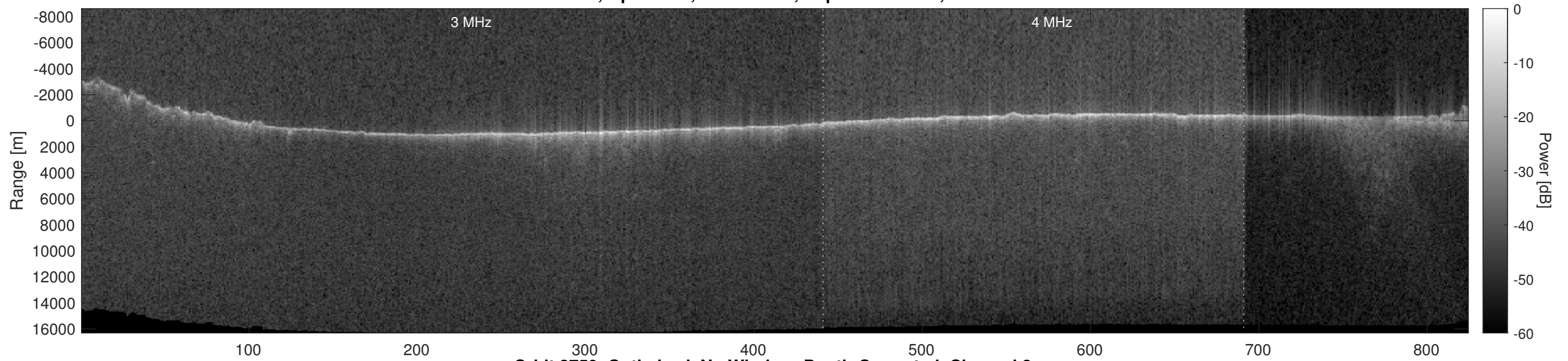
Orbit 3759, Optimized, No Window, Depth-Corrected, Channel 2
