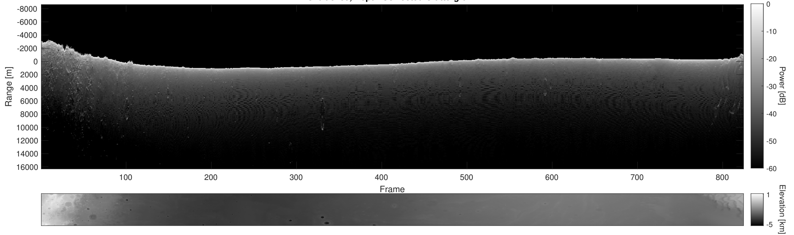
Orbit 3759, Depth-Corrected Cluttergram
