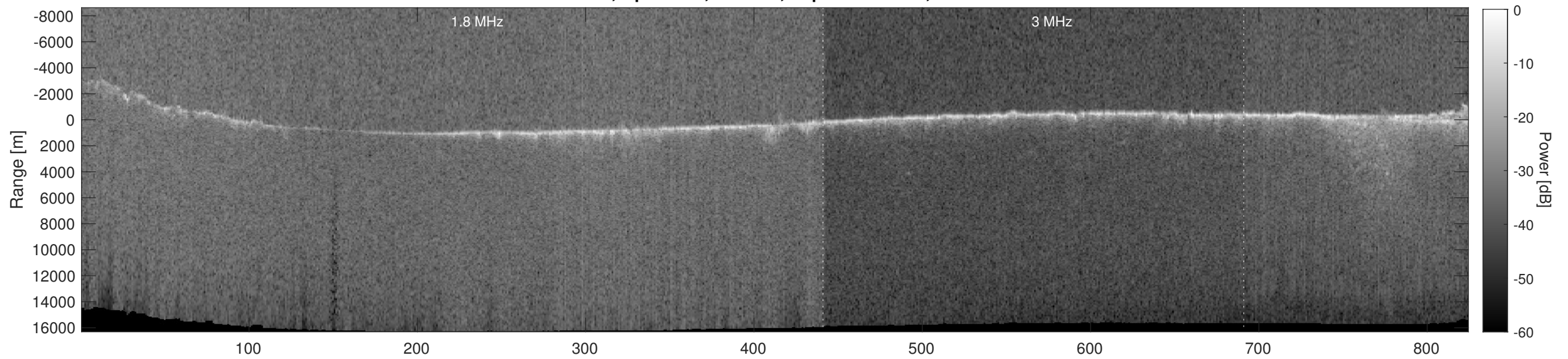
Orbit 3759, Depth-Corrected Cluttergram
