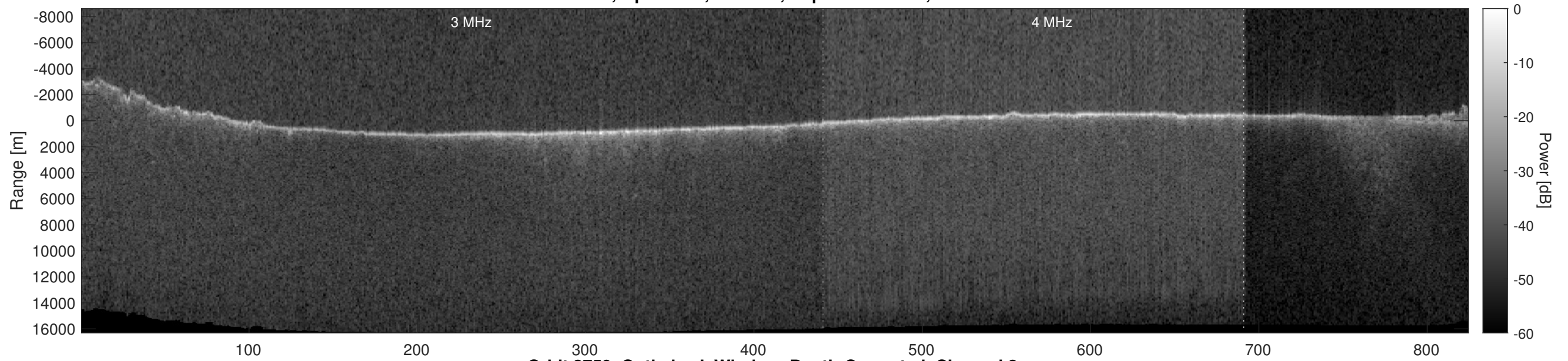
Orbit 3759, Optimized, Window, Depth-Corrected, Channel 2
