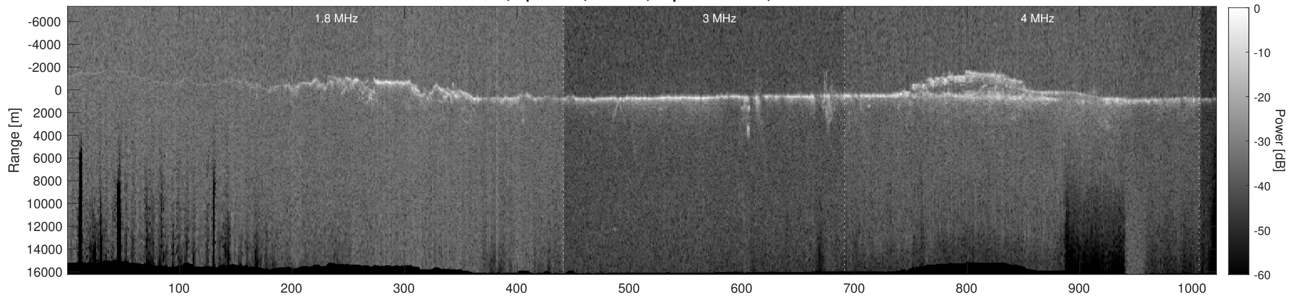
Orbit 3760, Depth-Corrected Cluttergram
