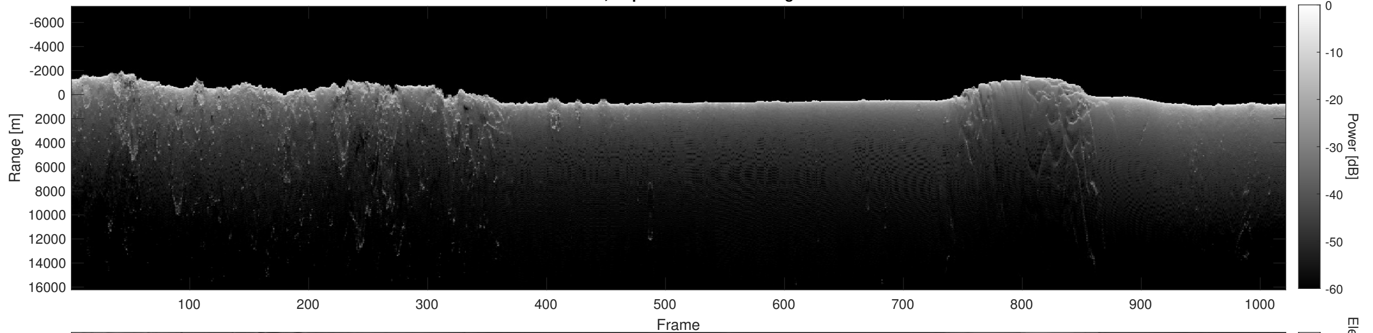
Orbit 3760, Depth-Corrected Cluttergram
