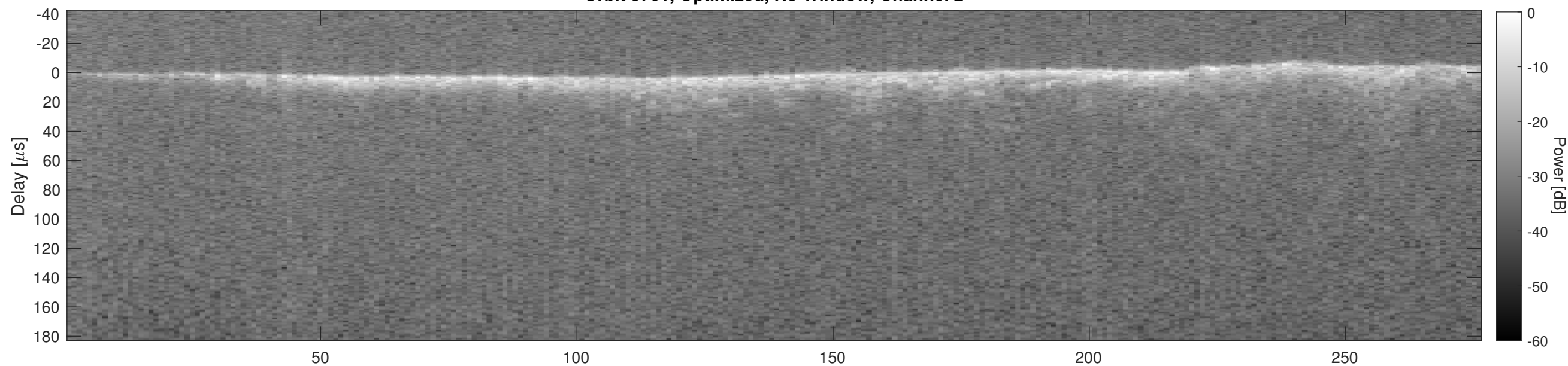
Orbit 3761, Cluttergram
