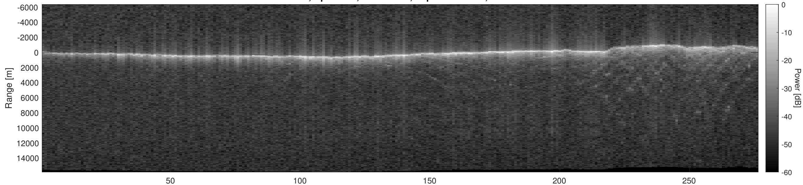
Orbit 3761, Optimized, No Window, Depth-Corrected, Channel 2
