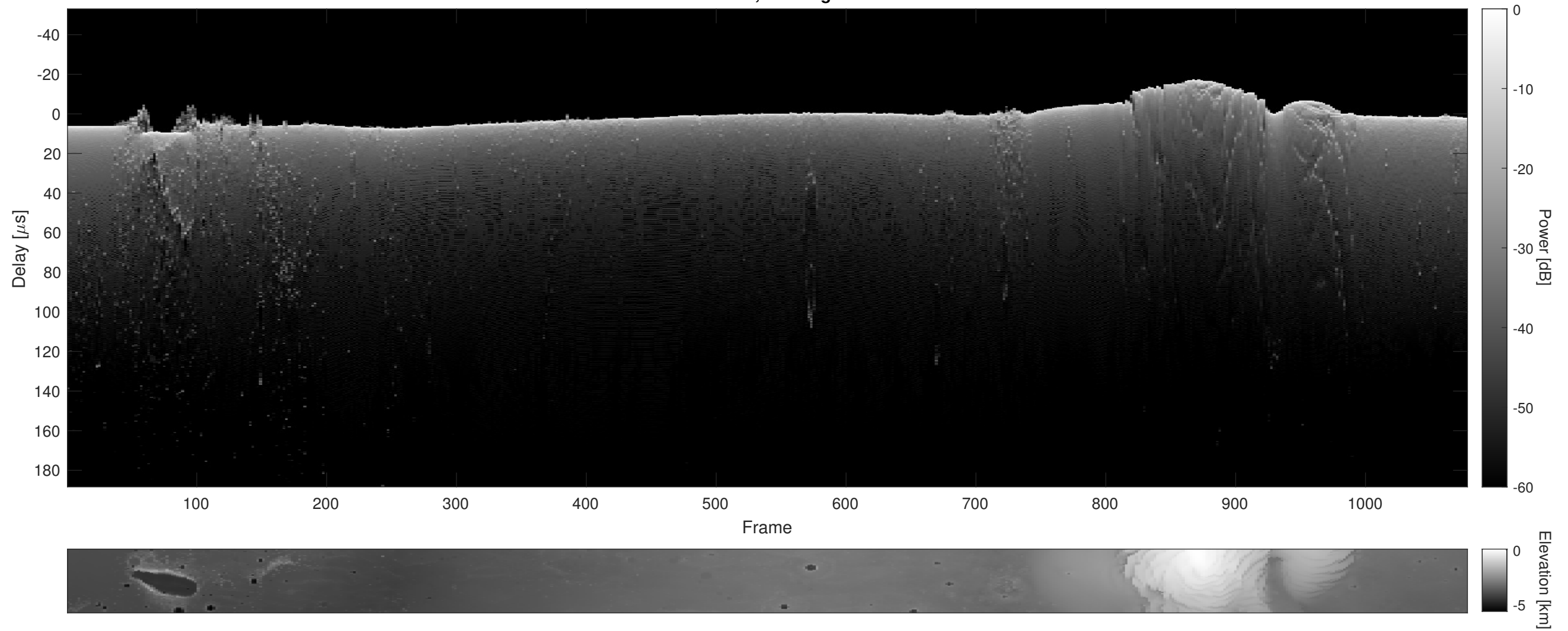
Orbit 3762, Cluttergram
